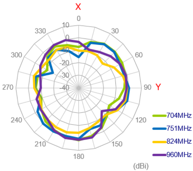
XY Plane
