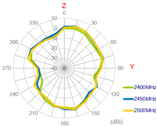
YZ Plane
