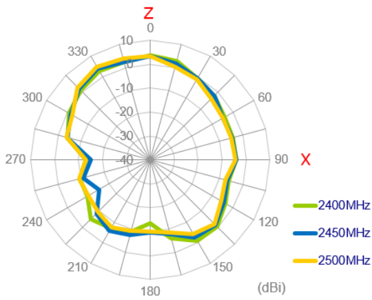
XZ Plane
